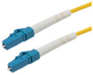
LC/UPC to LC/UPC Simplex 2mm Singlemode Patch Cord | 123-F1S1-3A566 | 123e.com Part Number: 123-F1S1-3A566
